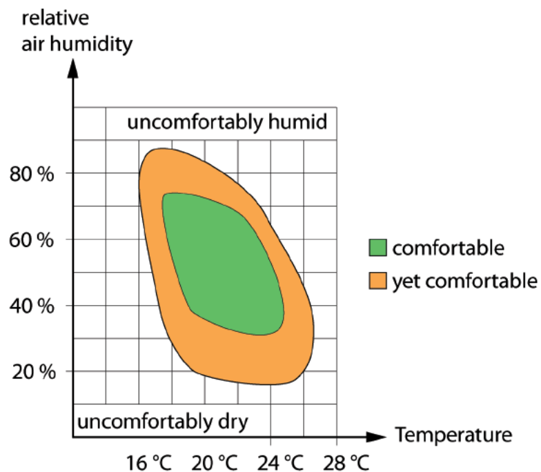
Figure 24: Comfort curve
