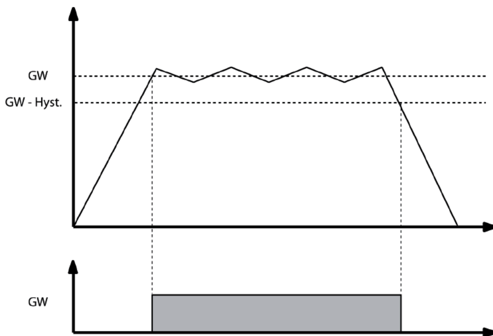
Figure 27: Frequency of switching with hysteresis parameterised.
