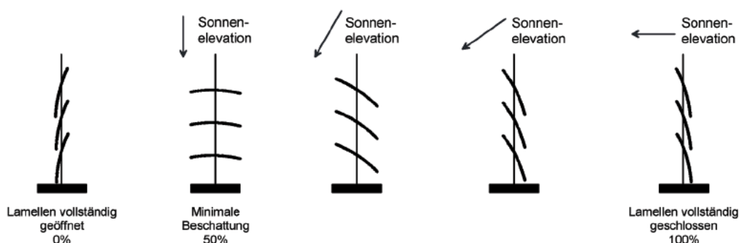
Figure 21: Slats are positioned according to the sun position
