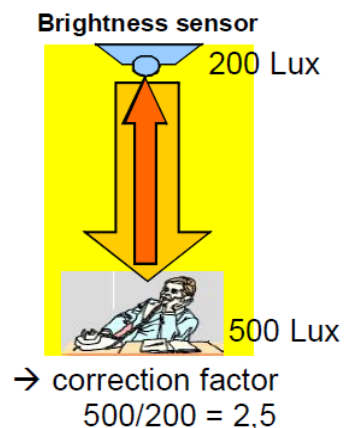
Fig. 8 Indirect measuring
