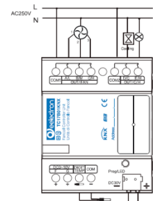
Wiring diagram for different configurations
