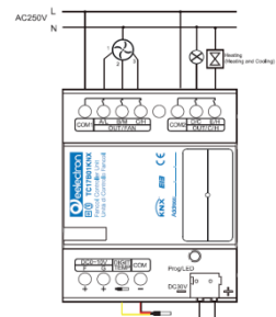
Wiring diagram for different configurations
