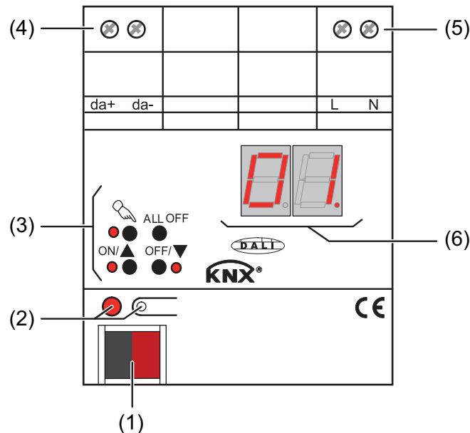
Figure 1: Device components
