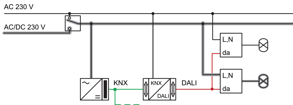
Figure 5: Electrical connection diagram in an emergency lighting system - KNX power supply and DALI emergency lights integrated into the emergency power supply
